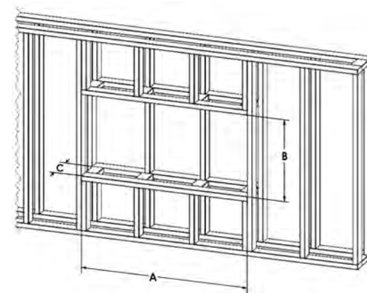
Rough Opening Fully Recessed
